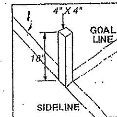
PYLON DETAIL
