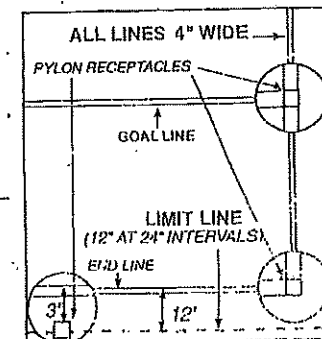
END ZONE DETAIL
